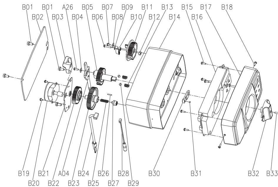
Bnt165PowerheadAssembly
