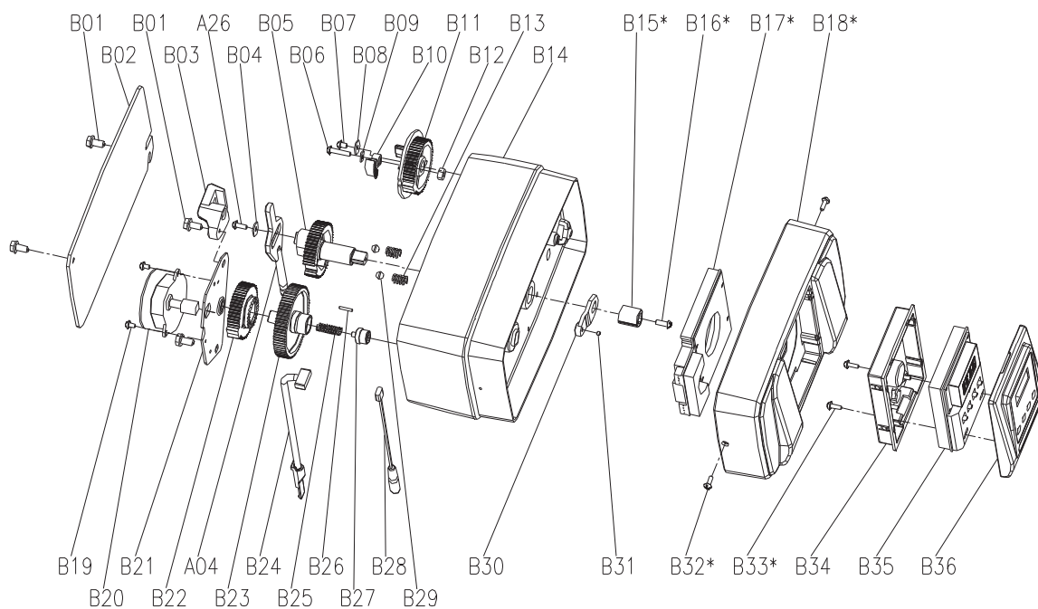
Bnt265PowerheadAssembly
